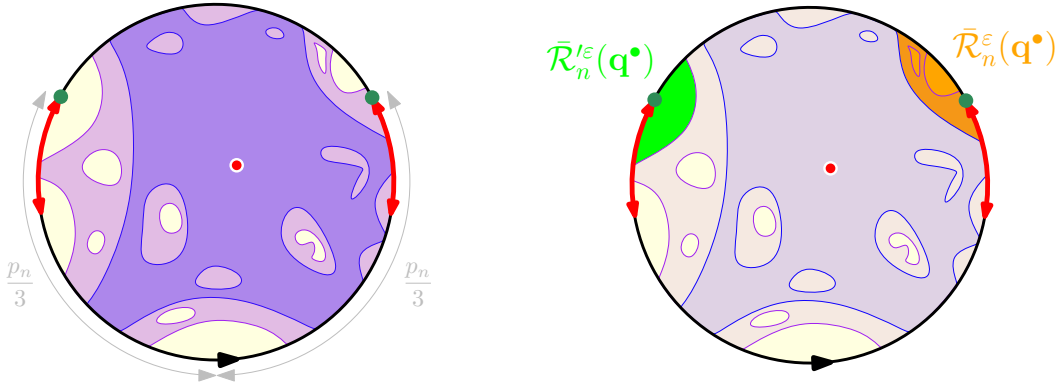
Fig 9: Definition of a second notion of restriction \mathcal{R}_n^{\prime\epsilon} , going “backwards” along the boundary. The ball used in the definition of \mathcal{R}_n^{\epsilon}(\mathbf{q}^\bullet) is depicted in purple with a blue outline. The (larger) ball involved in the definition of \mathcal{R}_n^{\prime\epsilon}(\mathbf{q}^\bullet) is in mauve. The difference between the map \mathbf{q}^\bullet and its restriction \mathcal{R}_n^{\epsilon}(\mathbf{q}^\bullet) is the same as the difference between \mathcal{R}_n^{\prime\epsilon}(\mathbf{q}^\bullet) and \mathcal{R}_n^{\epsilon}(\mathcal{R}_n^{\prime\epsilon}(\mathbf{q}^\bullet)) , provided the complements \bar{\mathcal{R}}_n^{\epsilon}(\mathbf{q}^\bullet) and \bar{\mathcal{R}}_n^{\prime\epsilon}(\mathbf{q}^\bullet) are disjoint.
