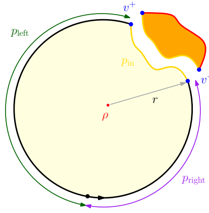
Fig 3: Notation for a restriction map. If the (n, \varepsilon) -restriction map \mathbf{r} appears as the restriction of a quadrangulation with area n' and perimeter p' , then the constraints (3.1) must be fulfilled.
