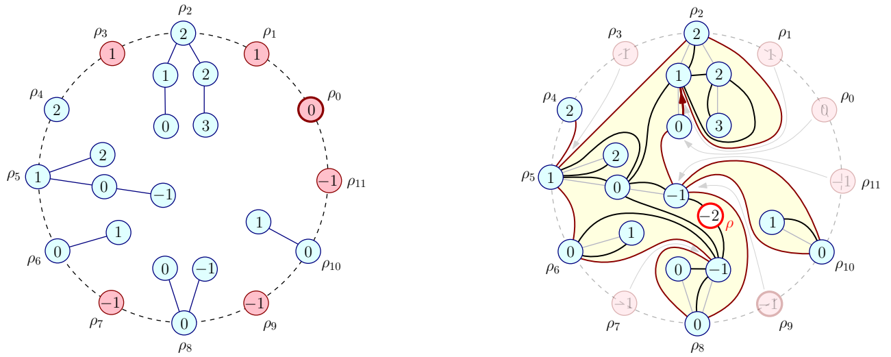
Fig 5: The bijection, from a labeled treed bridge to a pointed quadrangulation with a boundary. On this example, p = 12 , m = 11 , \lambda_* = -2 ; the tree with root vertex \rho_4 is a one-vertex tree. The edges of the cycle are dashed; its root \rho_0 has a thicker outline. The red vertices precede upsteps in the discrete bridge; they are not vertices of the output map. The gray arrows highlight the correspondence between the cycle and the boundary.
