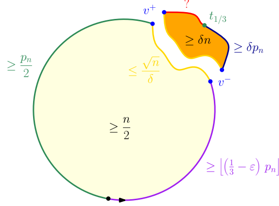
Fig 4: Inequalities defining (n, \delta) -good (n, \varepsilon) -restriction maps. The length of the red part of the boundary depends on the map of which the restriction map is the restriction. If this map has perimeter p_n , then the length of this red part is between \delta p_n and p_n .
