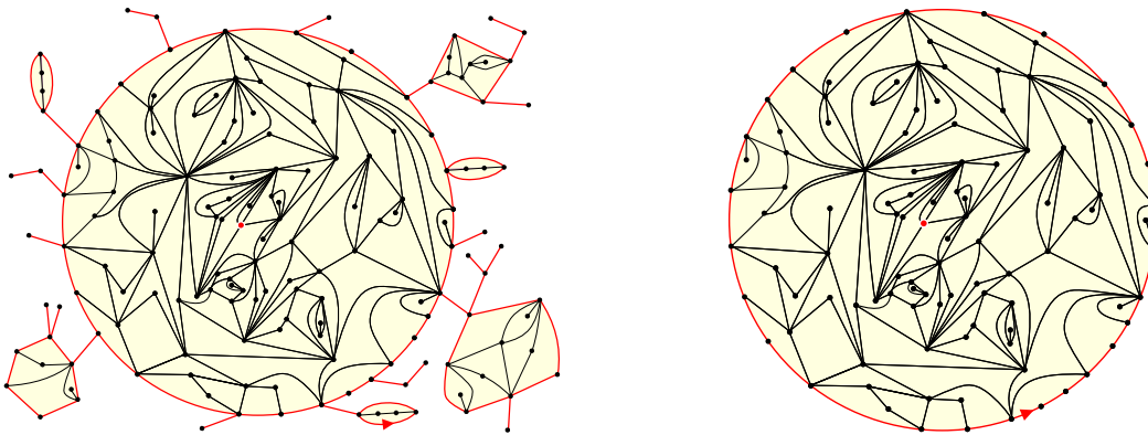
Fig 1: Quadrangulation with a boundary on the left; quadrangulation with a simple boundary on the right. The boundary is represented in red. These maps are pointed in the sense that a vertex, in red, is distinguished. The map on the right is in fact the so-called core of the pointed map on the left, defined in Section 2.1.
