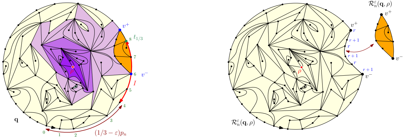
Fig 2: Definition of the restriction. We consider the smallest ball that hits the boundary of the map at boundary length between (\frac{1}{3} - \varepsilon)p_n and p_n/3 from the root. On this example, p = 26 , \lfloor (\frac{1}{3} - \varepsilon)p_n \rfloor = 4 , \lfloor p_n/3 \rfloor = 8 and r = 3 . The balls of radius 1 to 3 are depicted with lighter and lighter shades of purple. The restriction \mathcal{R}_n^\varepsilon(\mathbf{q}, \rho) is the map consisting of this ball with the addition of the (light yellow) components that do not contain t_{1/3} ; the so-called complement 5 \bar{\mathcal{R}}_n^\varepsilon(\mathbf{q}, \rho) is the (orange) component that contains t_{1/3} .
