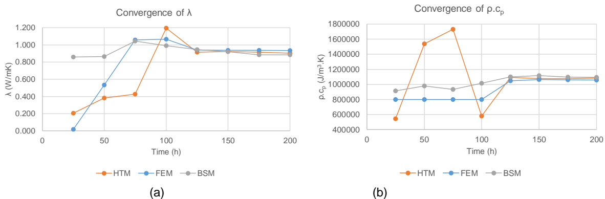
Figure 6- Convergence of the thermal conductivity \lambda (a) and the heat capacity \rho c_p (b) for the three numerical methods
