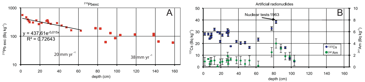
Fig. 5. Radionuclide dating of core CS03. (A): Profiles of 210 Pb exc activities (Bq kg -1 , dry weight) with depth in cm. The regression line between the top and 65 cm depth corresponds to an average sedimentation rate of 2.0 cm yr -1 . Deeper in the core the regression line corresponds to 3.8 cm yr -1 . (B): Profiles of artificial radionuclides 137 Cs and 241 Am activities (fallout from nuclear weapon testing) with depth in cm. The maximum activity at 83 cm depth for both nuclides corresponds to the maximum global fallout peak in 1963. Vertical bars for error.
