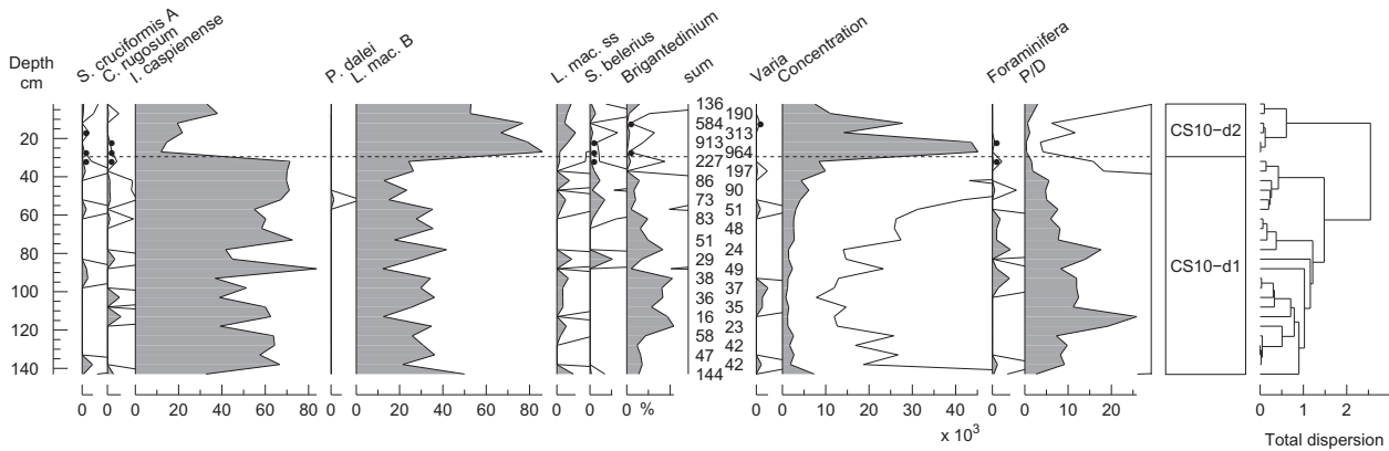
Fig. 6. Dinocyst diagrams of cores US01, US02, CS03 and CS10, taken in the south basin of the Caspian Sea. Concentration in numbers of dinocysts per ml of wet sediment. With 10x exaggeration curve. To the right dendrograms used for the zonation.
