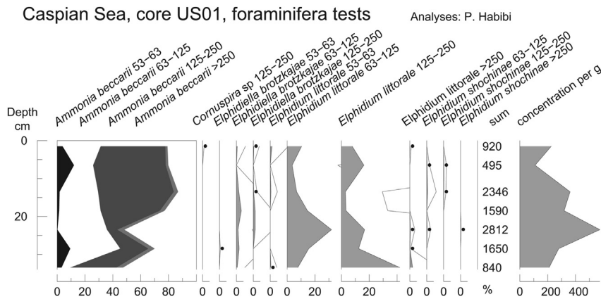
Fig. D1. Foraminiferal assemblages of core US01, taken in the south basin of the Caspian Sea. Names with fraction size in \mu\text{m} .
