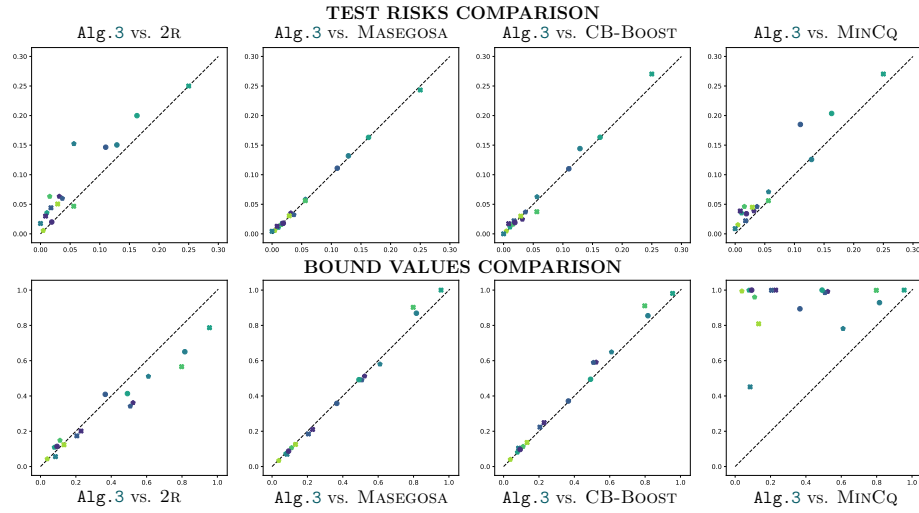
FIGURE 1: Pairwise comparisons of the test risks (first line) and the bounds (second line) between Algorithm 3 and the baseline algorithms. Algorithm 3 is represented on the x-axis, while the y-axis is used for the other approaches. Each dataset corresponds to a point in the plot and a point above the diagonal indicates that Algorithm 3 is better.
