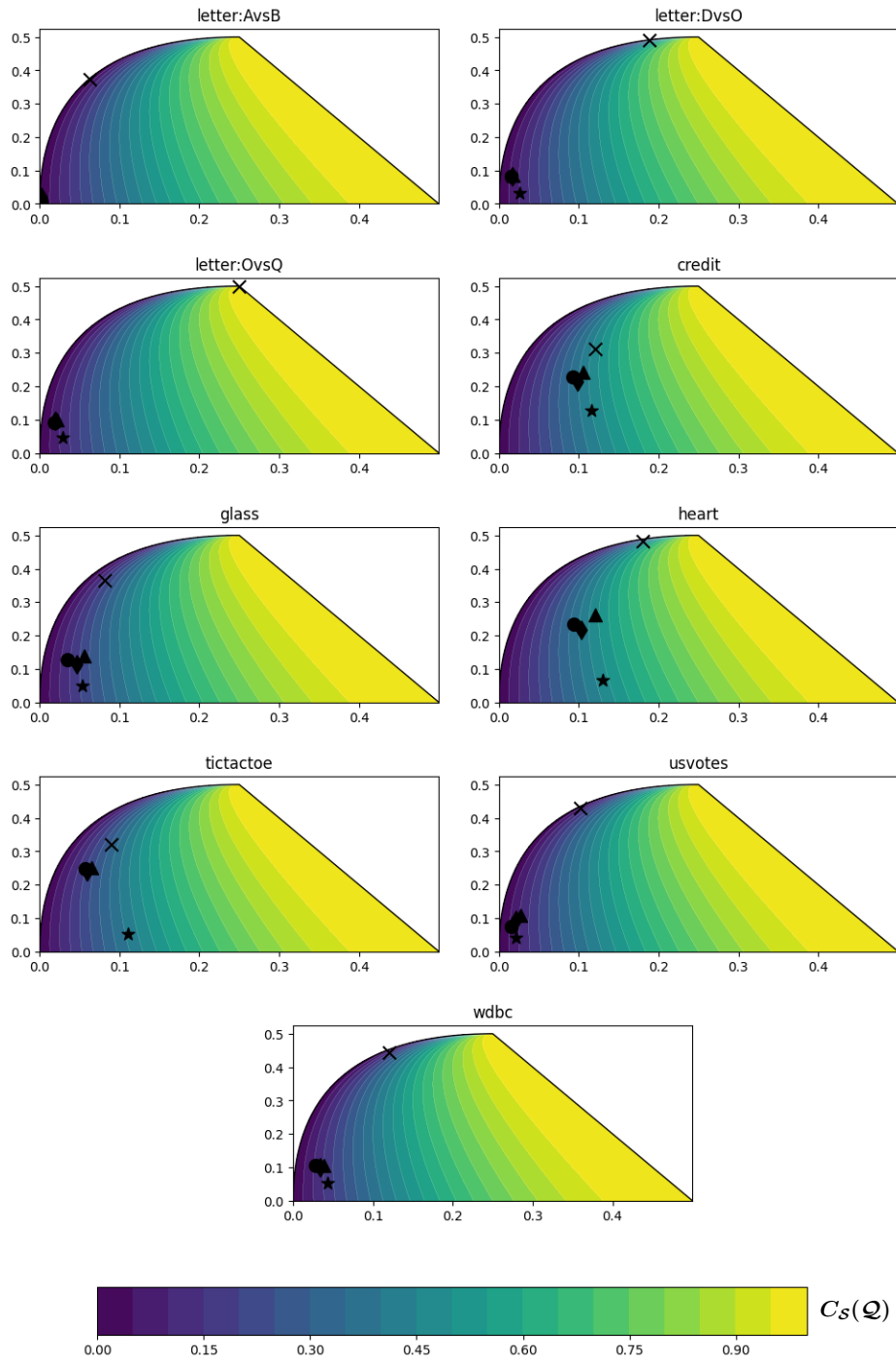
FIGURE 3: Representation of all the possible values of the empirical C-Bound C_S(Q) in function of the disagreement d_S(Q) (y-axis) and joint error e_S(Q) (x-axis). We report the values obtained on different datasets by Alg.3 (◆), MASEGOSA (▲), 2R (★), CB-Boost (●), and MinCq (×).
