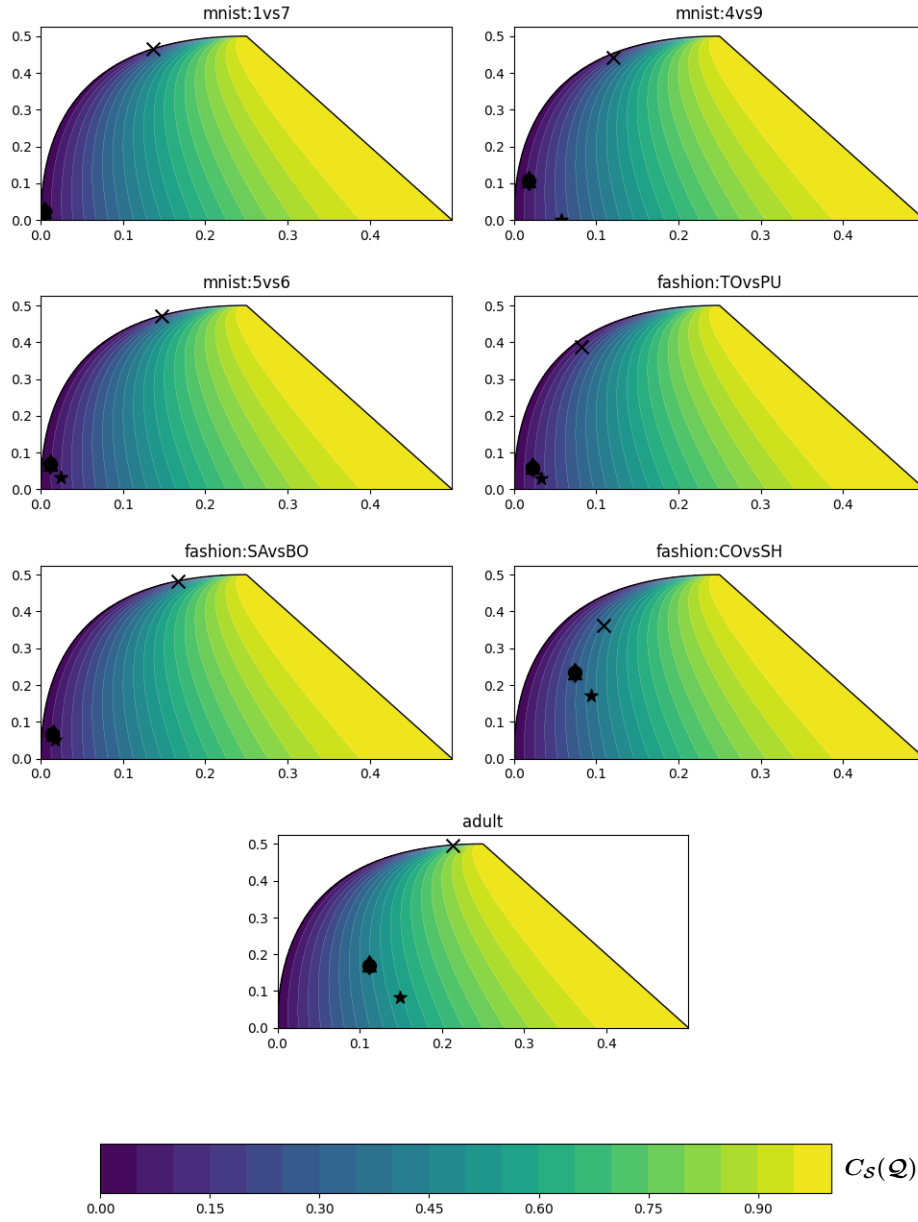
FIGURE 2: Representation of all the possible values of the empirical C-Bound C_S(\mathcal{Q}) in function of the disagreement d_S(\mathcal{Q}) (y-axis) and joint error e_S(\mathcal{Q}) (x-axis). We report the values obtained on different datasets by Alg. 3 ( \blacklozenge ), MASEGOSA ( \blacktriangle ), 2R ( \blackstar ), CB-Boost ( \bullet ), and MinCq ( \times ).
