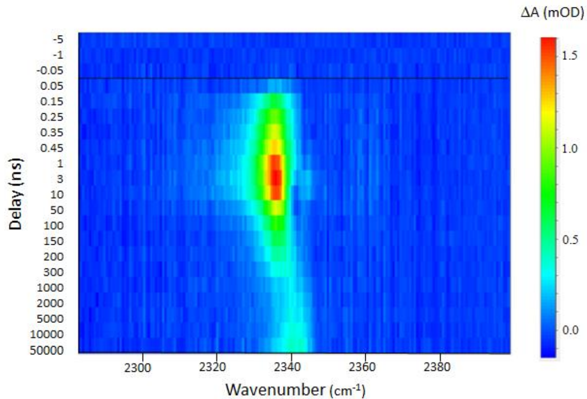
2 Fig. S9: Formation of CO 2 co-product studied by TR-IR.
