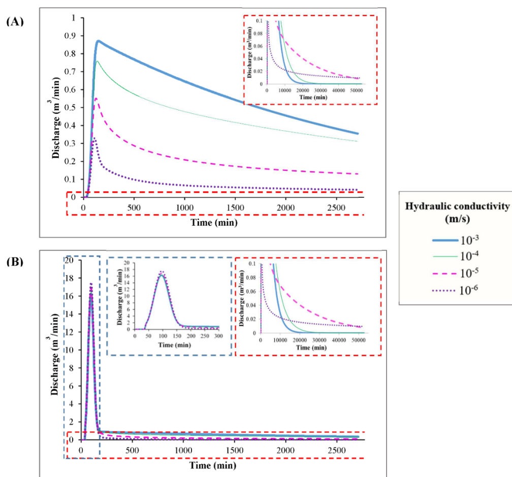
Figure 7. Spring hydrograph variability in relation to matrix hydraulic conductivity changes in scenarios A3 (A) and B3 (B).
