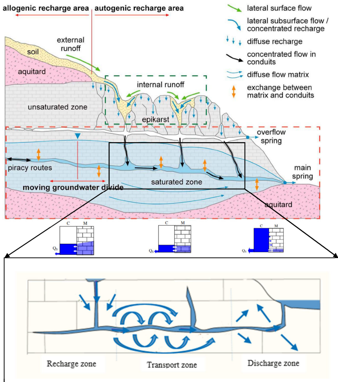
Figure 1. Conceptual model of flow in the karst aquifer with the dual-porosity (modified from Bailly-Comte et al. [16], Hartmann et al. [3], Binet et al. [33]).
