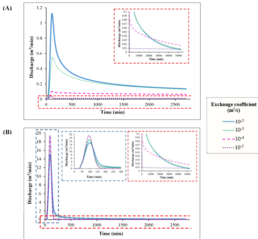
Figure 4. Spring hydrograph variability in the relation to the exchange coefficient changes in scenarios A1 (A) and B1 (B).
