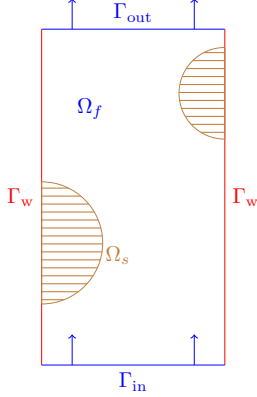
Fig. 1: Sketch of \Omega
