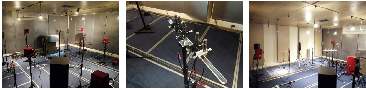
Figure 4 Picture of the acoustic lab. From left to right: the overall setup, one microphone array, the setup with revolved panels.
