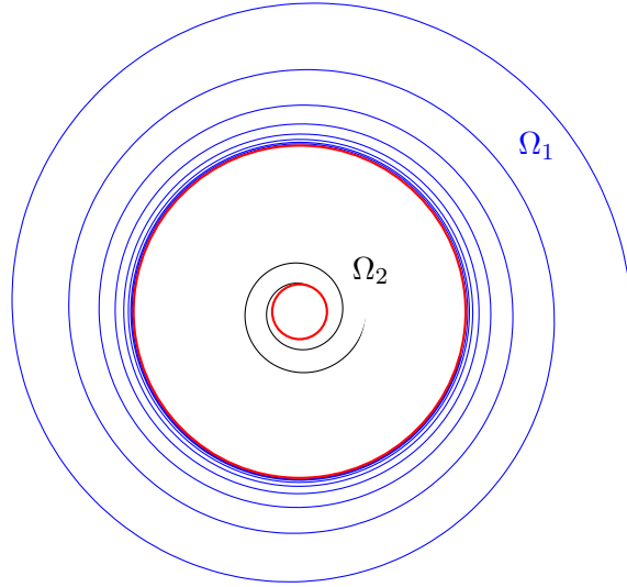
FIGURE 2. Example of a situation that might happen in Theorem 4.2 where \Omega_1 and \Omega_2 are outer snakes with no common point.
