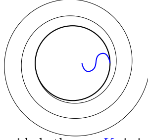
FIGURE 1. Case avoided: the arc K_j is in the bounded component of \overline{K_i}^c where K_i is the outer snake
