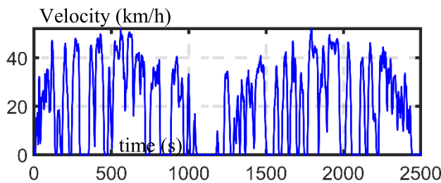
FIGURE 9. Urban driving cycle.
