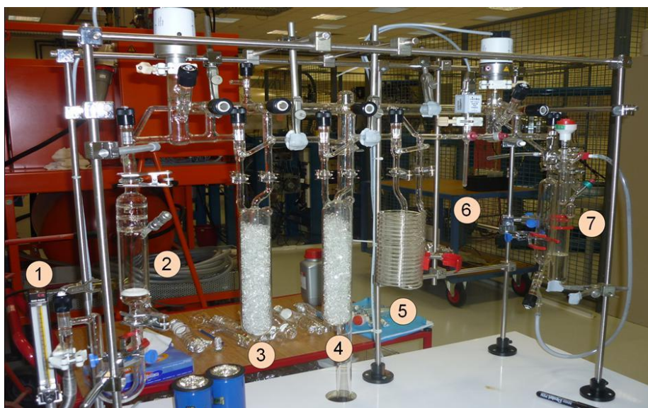
Figure 1 Photograph of the DIC extraction line. 1: the flowmeter; 2: stripping vessel; 3, 4, 5: cold traps (respectively at 80^{\circ}\text{C} , 80^{\circ}\text{C} , and 190^{\circ}\text{C} ); 6: cold finger with a MKS gauge; 7: 2 aliquots in 2 different vials. Vacuum is generated by a dry primary pump coupled to a turbopump. Residual pressure is measured by 2 full range Pfeiffer gauges.
