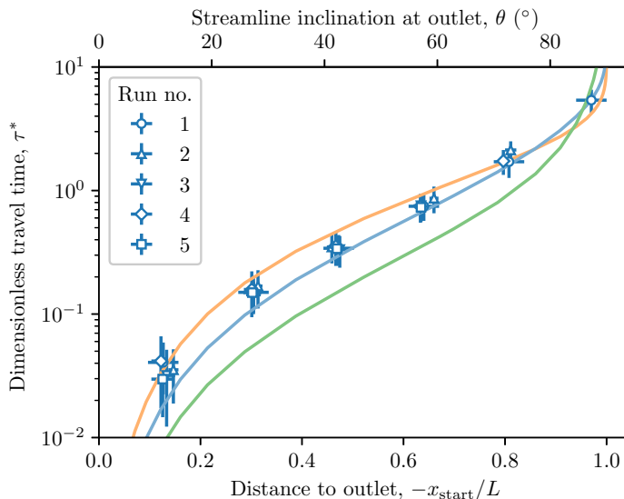
Figure 9: Dimensionless travel time of a parcel of dye, \tau^* , as a function of the distance to the outlet -x_{\text{start}}/L (lower axis). Upper axis: streamline inclination at the outlet, \theta . Blue markers: experimental runs (table 1). Vertical error bars indicate the exit duration, \Delta\tau/\langle\tau\rangle ; horizontal ones indicate initial width of the parcel. Colored lines: theoretical travel times after section 5.2 for aspect ratios a = 0.35 (green), 0.7 (blue, our laboratory experiment), and 1.4 (orange).
