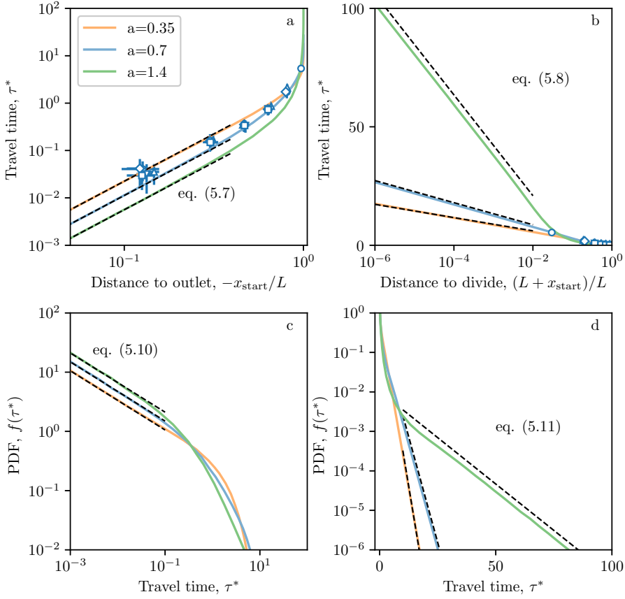
Figure 10: Travel times through a rectangle aquifer. (a) and (b) Dimensionless travel time, \tau^* , as a function of distance to outlet, -x_{\text{start}}/L , and distance to divide, (L + x_{\text{start}})/L . Colored lines: theoretical travel times, after section 5.2. Black dashed lines: asymptotic regimes (5.7) and (5.8). Blue markers: experimental data (same symbols as in figure 9), vertical error bars indicate the exit duration, \Delta\tau/\langle\tau\rangle , horizontal ones indicate the initial width of the parcel. (c) and (d) Probability density functions (PDF) of travel times, f(\tau^*) , for several aspect ratios. Black dashed line: asymptotic regimes (5.10) and (5.11).
