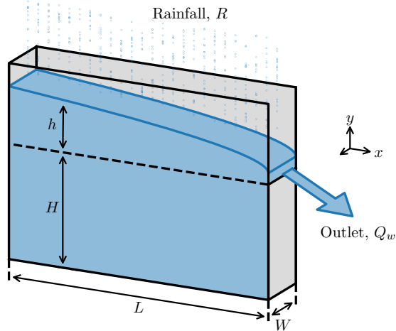
Figure 1: Experimental setup and notations. The aquifer is made of glass beads (shaded area) piled between two vertical glass plates (black solid lines) separated by a gap of width W = 5 cm. Its length and depth are L = 90 cm and H = 62 cm, respectively. A series of 24 capillary tubes (diameter 1.2 mm, length 50 cm) placed above the tank simulate rainfall, by distributing water uniformly over the aquifer's surface.
