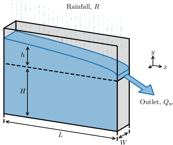
Figure 1: Experimental setup and notations. The aquifer is made of glass beads (shaded area) piled between two vertical glass plates (black solid lines) separated by a gap of width W = 5 cm. Its length and depth are L = 90 cm and H = 62 cm, respectively. A series of 24 capillary tubes (diameter 1.2 mm, length 50 cm) placed above the tank simulate rainfall, by distributing water uniformly over the aquifer's surface.
