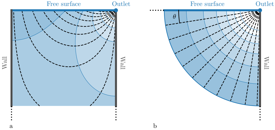
Figure 7: (a) Flow in an infinitely deep aquifer. (b) Asymptotic regime near the singularity at the aquifer outlet. Black dashed line : streamlines (linearly spaced), blue shading : hydraulic head. \theta : inclination of the streamlines with respect to horizontal.
