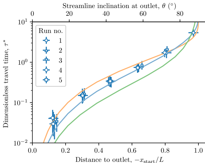
Figure 9: Dimensionless travel time of a parcel of dye, \tau^* , as a function of the distance to the outlet -x_{\text{start}}/L (lower axis). Upper axis: streamline inclination at the outlet, \theta . Blue markers: experimental runs (table 1). Vertical error bars indicate the exit duration, \Delta\tau/\langle\tau\rangle ; horizontal ones indicate initial width of the parcel. Colored lines: theoretical travel times after section 5.2 for aspect ratios a = 0.35 (green), 0.7 (blue, our laboratory experiment), and 1.4 (orange).
