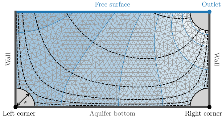
Figure 8: Mesh (grey triangles) of an aquifer skirting the two stagnation points and the aquifer outlet (grey disks). Black dotted lines : streamlines (logarithmically spaced). Blue shading : hydraulic head. The aquifer aspect ratio is a = 0.5 . For illustration, we set the radius of the quarter circles to \epsilon/L = 0.1 and the maximum mesh size to \delta\ell/L = 0.025 . In practice, travel times are calculated with \epsilon/L = 0.05 and \delta\ell/L = 0.0125 .
