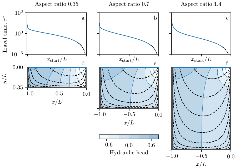
Figure 6: Steady-state flow in aquifers of aspect ratio a = 0.35, 0.7 (as in our laboratory experiment), and 1.4 , respectively, after equation (4.11). (a-c) Dimensionless travel time of rainwater, \tau^* , as a function of relative landing position, x_{\text{start}}/L . Solid blue line : numerical approximation (section 5.2). Black dashed line : expansion near the outlet, equation (5.2). (d-f) Streamlines (black dashed lines) and hydraulic head (blue shading).
