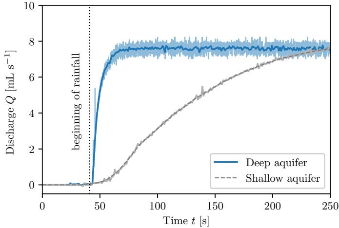
Figure 2: Discharge at the outlet of our deep experimental aquifer (blue line) and of a shallow one (black dashed line, Guérin, 2015). Light color: raw signal, dark color: average over 10 successive data points. Vertical dotted line: beginning of rainfall. Both aquifers are 5 cm wide and 90 cm long; they are made of the same 1 mm glass beads, and are submitted to similar rainfall inputs: Q_{\text{in}} = 7.9 \text{ mL s}^{-1} for the deep aquifer and 8.3 \text{ mL s}^{-1} for the shallow one.
