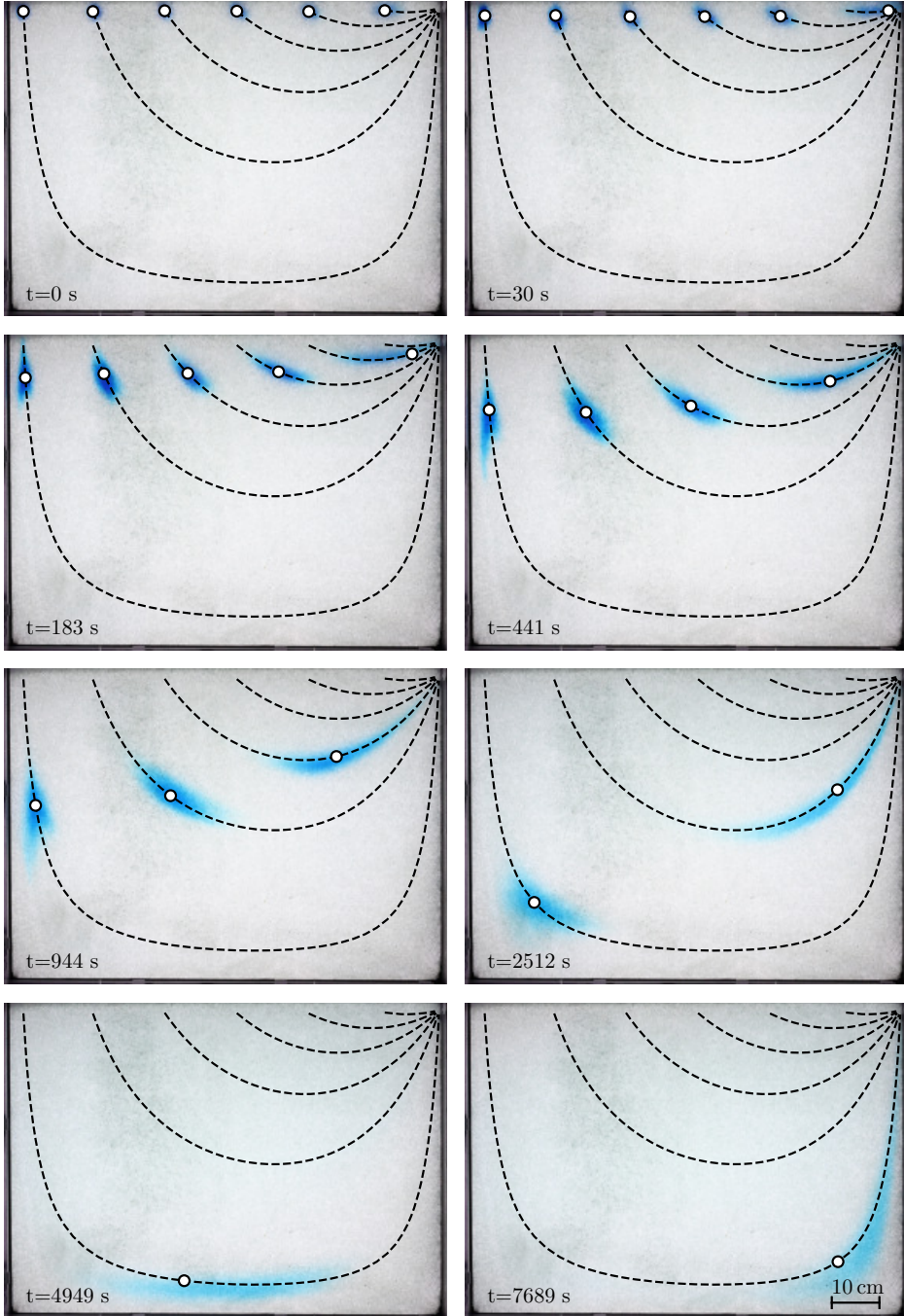
Figure 3: Propagation of parcels of dye through the aquifer during run no 1 (table 1, time indicated on each snapshot). Dye parcels are injected through the surface of the aquifer at distance \ell = 87.3, 72.7, 57.6, 42.5, 27.4, and 11.4 cm from the outlet. The aquifer, made of 3 mm glass beads, receives a rainfall input Q_{in} = 6.3 \text{ mL s}^{-1} . Black dashed lines: streamlines after equation (4.11). White dots: position of the dye parcels after equation (5.1). Theory has no adjustable parameters.
