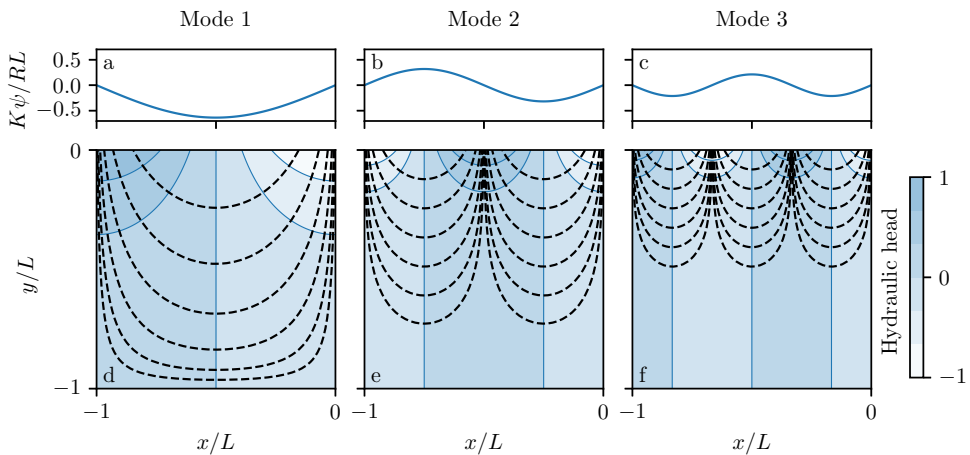
Figure 5: First three modes of the complex velocity potential (4.11) in an aquifer of aspect ratio a = 1 . (a-c) Dimensionless stream function K\psi/(RL) at the free surface ( y = 0 ). (d-f) Streamlines (black dashed line) and hydraulic head (blue shading, normalized to 1).
