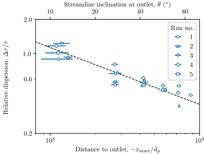
Figure 11: Relative dispersion, \Delta\tau/\tau , as a function of the distance to outlet rescaled with pore size -x_{\text{start}}/d_p (lower axis). Upper axis: streamline inclination near the outlet, \theta . Blue markers: experimental data (table 1). Black dashed line: equation (6.1) fitted to data.
