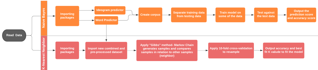
Figure 17: Knowledge Mining process flow
