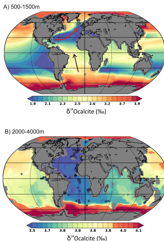
Fig. 10. Simulated ocean calcite \delta^{18}\text{O} (500–1500 m in (A) and 2000–4000 m in (B) ) for the present day with i LOVECLIM. Superimposed dots represent calcite- \delta^{18}\text{O} data measured on benthic foraminifer species (Marchal and Curry, 2008, extended by 73 points: Table S2). The North Atlantic drift (red arrow in A ) is well represented as the penetration of the Antarctic intermediate waters moving northward (black arrow in A ). Note that the legend is non-linear.
