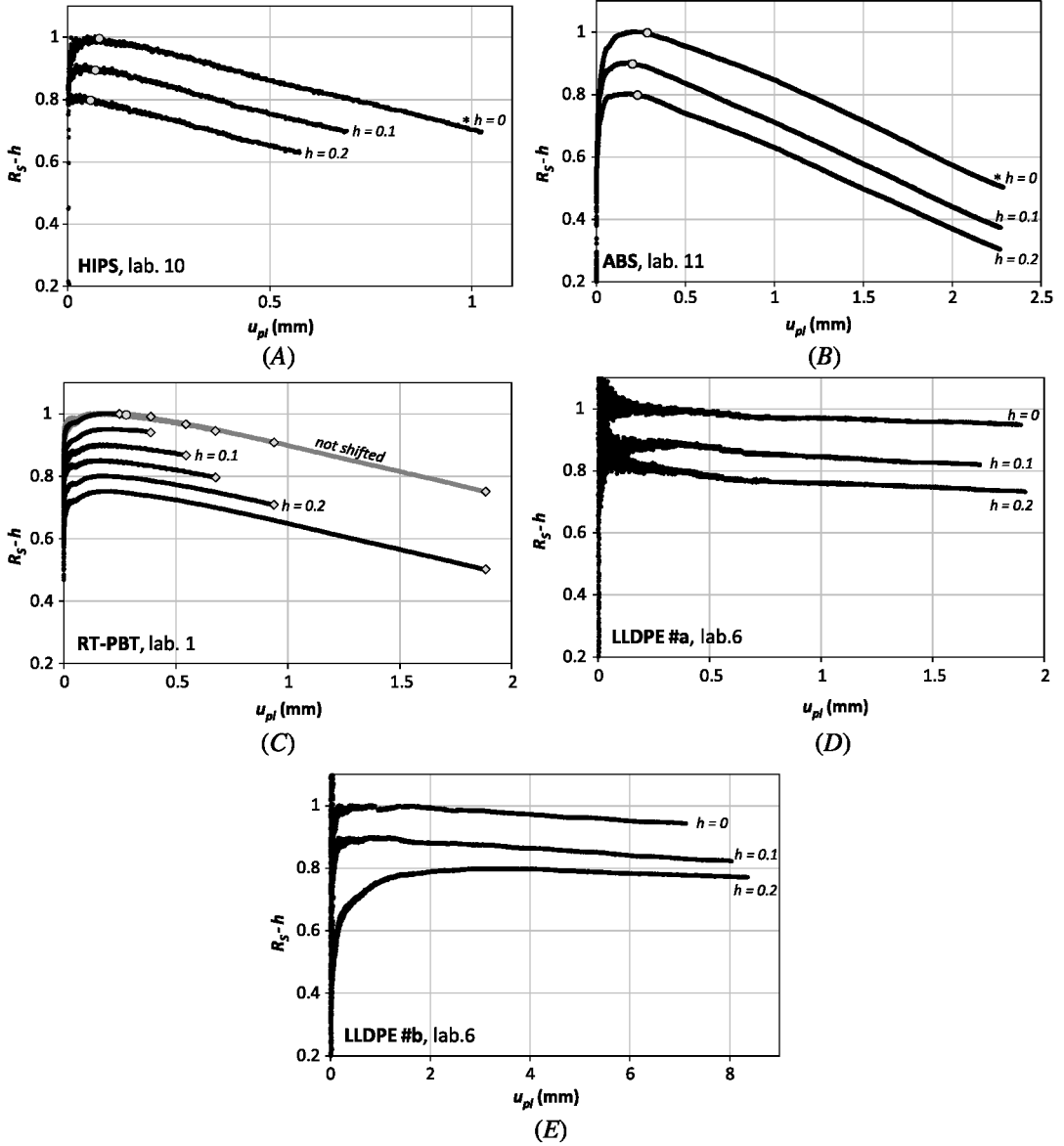
FIG. 3 R_S curves of different nominally identical sN specimens of (A) HIPS, from Laboratory 10; (B) ABS, from Laboratory 11; (C) RT-PBT, from Laboratory 1; (D) and (E) LLDPE, #a and #b, respectively, from Laboratory 6. The curves are vertically shifted by an h -factor. In (A), (B), and (C), the gray circles indicate the limit point. In (C), the curves are also represented as not shifted (in gray); rhomb indicates the final point (that is, the point at which the test was interrupted). See text for explanation of the asterisk in (A) and (B).
