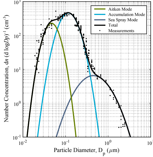
Figure 3. Number concentration size spectra measured from the PCASP-100X (0.1–3 \mu\text{m} ) and the DMPS (0.02–0.3 \mu\text{m} ) on February 20 th , 2018 at 1300 UTC. Particle sizes have been corrected to 80% relative humidity (Gerber, 1985). Number concentrations for particles larger than 0.5 \mu\text{m} were used to constrain a single log-normal number concentration size distribution (“SSP mode”). This method has been used by other researchers (e.g. Modini et al. (2015) and Quinn et al. (2017)) to constrain the contribution of SSPs to the total number concentration size spectra. The Aitken and accumulation modes are shown for reference.
