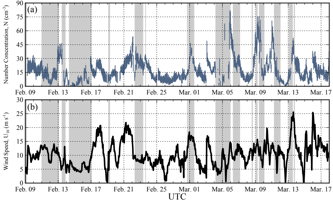
Figure 4. (a) The average hourly number concentration of sea spray particles is shown for the entire campaign with periods of fog ( \text{RH} > 98\% ) or rain ( > 1 \text{ mm hr}^{-1} ) marked by the shaded areas. (b) The hourly 10 m wind speed.
