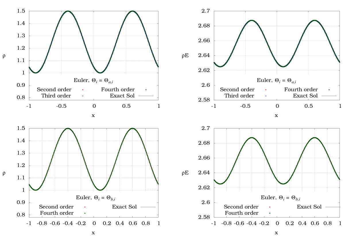
Fig. 4.2: Second-, third- and fourth-order accurate approximation of the smooth Euler solution and entropy with a mesh made of 400 cells.
