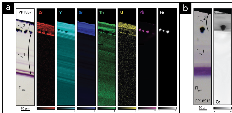
Figure 5. Transmitted plane-polarized light microphotographs and corresponding synchrotron radiation X-ray fluorescence elemental maps through a transect from the core crystal of Fl geo to the Fl og rim from (a) sample PP18S7 and (b) PP18S15. Black areas indicate a concentration below the limit of detection of the element. Globular pyrite crystals are included in Fl og2 .
