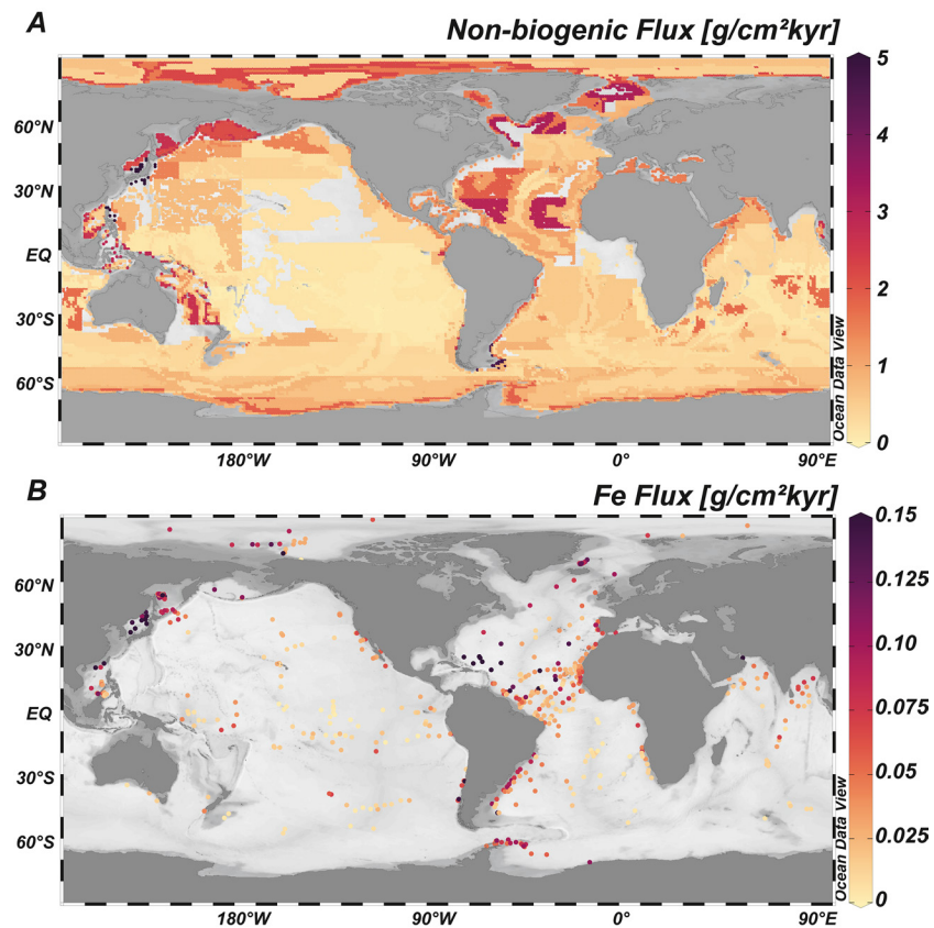
Figure 7. Th-normalized flux of (a) nonbiogenic material based on spatially interpolated mass flux and CaCO 3 , opal and organic matter observations and (b) Fe flux based on spatially interpolated mass flux and discrete Fe observations.
