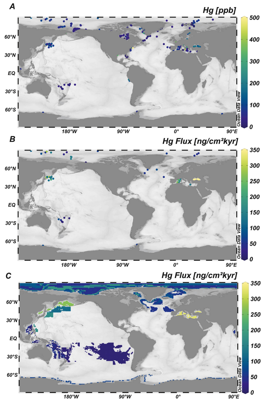
Figure 8. (a) Hg concentrations, (b) flux of Hg in surface sediments extrapolated using discrete Hg observations, and (c) flux of Hg using spatially-interpolated Th-normalized flux and zone-averaged Hg observations. Note in many cases here a limited number of observations are interpolated across relatively large interpolation zones, for example, in the South Pacific Subtropical Gyre and around Antarctica.
