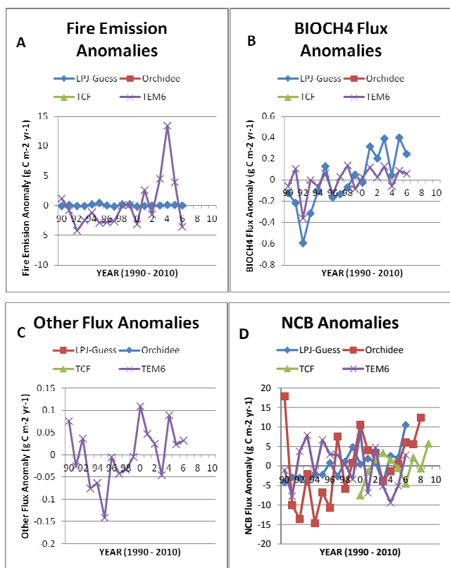
Fig. 6. Comparisons among LPJ-Guess, Orchidee, TCF, and TEM of inter-annual variability between 1990 and 2010 for anomalies of fire emissions (Panel A), biogenic CH 4 emissions (Panel B), Other fluxes (harvest and DOC exports, Panel C), and net carbon balance (NCB, Panel D).
