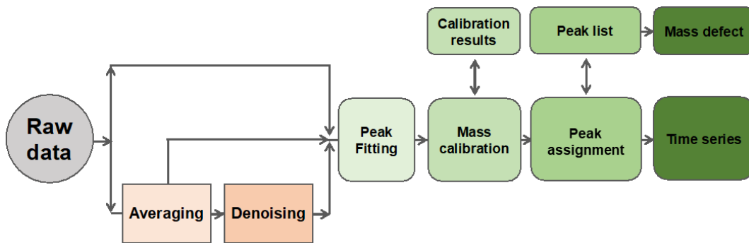
Figure 1: Simplified schematics of the working principle of Orbitool.
