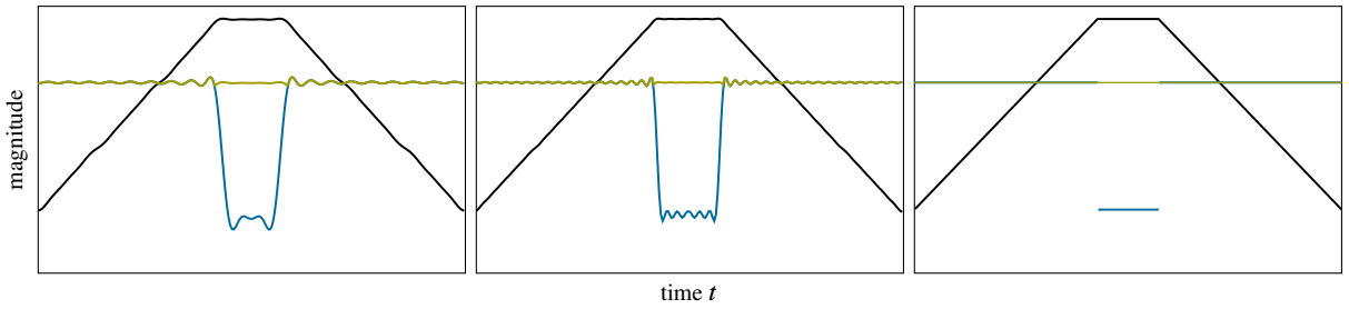
Figure 6: Boundary displacement u(1, t) [—] and strain u_x(1, t) [—] along with Signorini residual r [—] for a periodic solution with active contact: m = 20 [left], m = 40 [center] and exact solution [right].
