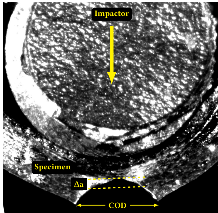
Figure 7 Details of the blunted crack tip during the deformation; measurements of the Crack Opening Displacement and the crack extension ( \Delta a ).
