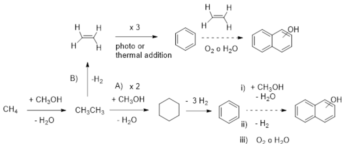
Fig. 6. Formation pathways of oxy-PAHs. A: Sequential FTT process involving methane and methanol followed by radical ring-closure dehydrogenation and terminal oxidation. B: FTT process involving methane and methanol to yield ethene followed by sequential thermal or UV cyclization and final oxidation.
