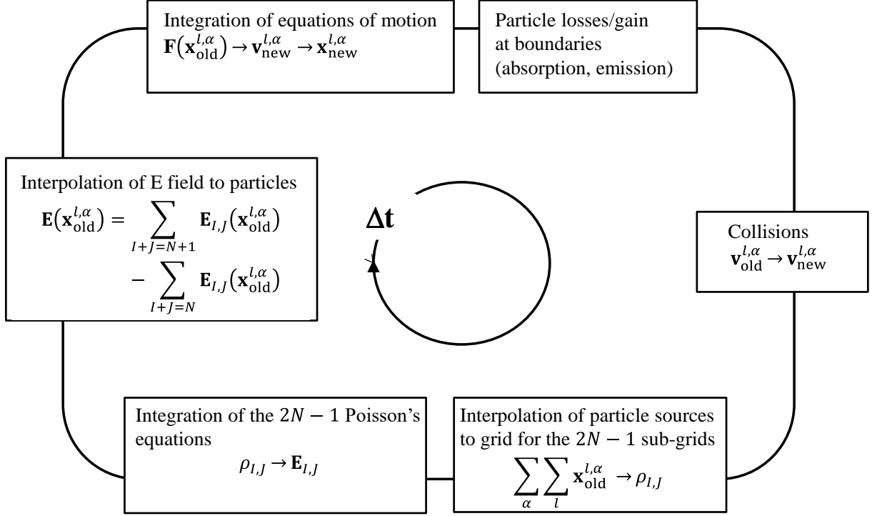
Figure 2: Sparse PIC algorithm. The indices l and \alpha refer to a given particle l of specie \alpha .
