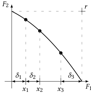
Figure 8: Illustration of the reparametrization of a set of p points of the Pareto front by \delta .
