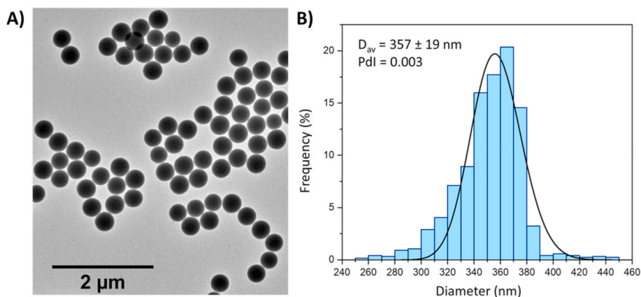
Fig. 3. A) TEM image and B) size distribution of initial silica nanoparticles (Np).
