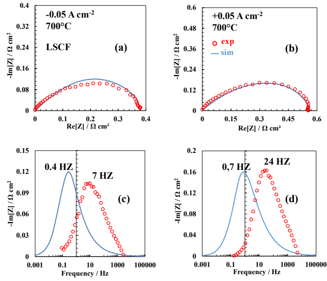
Fig. 6. Experimental and simulated impedance diagrams for the LSCF electrode at 700°C for i_{dc} = \pm 50 \text{ mA cm}^{-2} . (a) and (b) Nyquist and (c) and (d) Bode plots.
