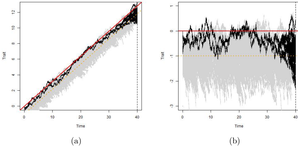
Figure 1: Ancestral lineages of the present population. To an individual of trait x living at time T , its lineage corresponds to the function that associates with each time t < T the trait of this individual if it was already born, or else the trait of its closest ancestor at that time (its parent if the latter was born, otherwise its grand-parent etc.). The traits in the population (ordinate) are shown with respect to time (abscissa). The extinct lineages are in gray, whereas the lineages of the living particles are in black. As can be seen, the trait distribution is nearly stationary (gray background on the right image), whereas the lineages follow an Ornstein-Uhlenbeck process (see our main result, Theorem 1.1). (a): fixed frame. (b): moving frame. The parameters are c = 1 , \sigma = 0.32 , K = 250 .
