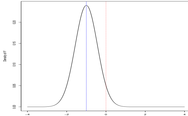
Figure 2: Density of the stationary solution F of (2). The mode of this density is -c = -1 here, and the variance of F is \sigma = 0.32 , so that \lambda = 0.34 .
