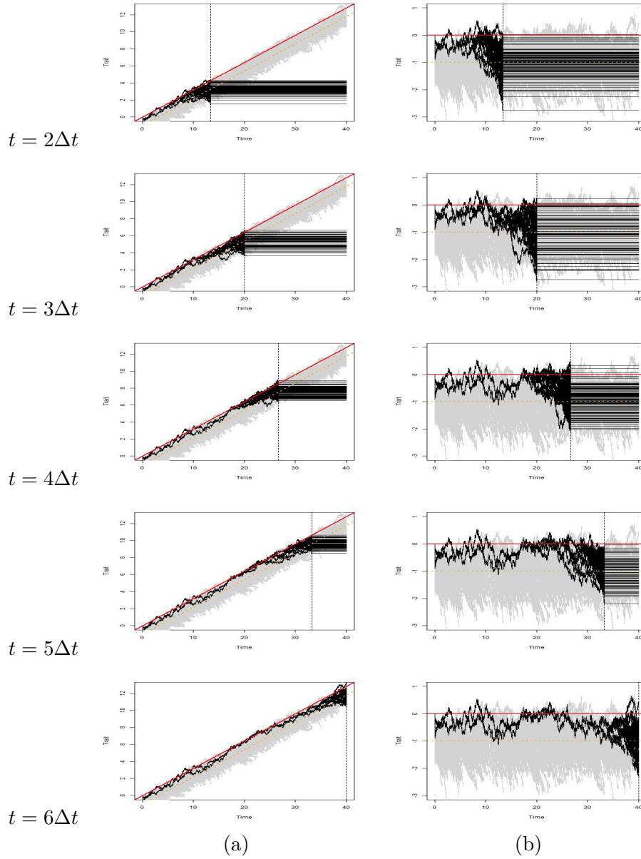
Figure 3: Evolution of the ancestral lineages of the present population, for various times t = k\Delta t with \Delta t = 20/3 and k \in \{2, \dots, 6\} . The traits in the population (ordinate) are shown with respect to time (abscissa). The extinct lineages are in gray, whereas the lineages of the living particles are in black. (a): fixed framework. (b): mobile framework.
