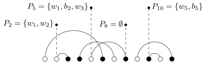
FIGURE 2. The stack of a matching at position i is given by all the points on the left side of point i (including i itself) that are matched to a point on the right side of point i . In the picture, w_i is the i -th white point from the right, and analogously b_i is the i -th black point from the right. At the locations specified by the dashed lines, we show the stack of the represented matching.
