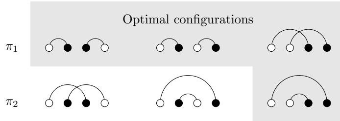
FIGURE 1. Optimal matchings at p = 1 for 2N = 4 points. \pi_1 is the matching in which the first white point is matched with the first black point; \pi_2 is the only other possible matching. All optimal configurations satisfy k_\pi(x) = k_{\text{LB}}(x) .
