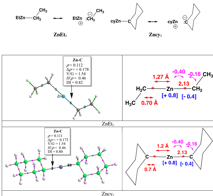
Fig. 9 (Left) QTAIM molecular graph calculated for \text{ZnEt}_2 and \text{ZnCy}_2 . Bond critical points are located as small magenta spheres, zinc atom in grey, carbon atoms in green and hydrogen atoms in white colour. (Right) Schematic map of selected ELF attractors (red stars), displaying in red their average populations (in e ), covariance values in magenta and QTAIM atomic charges in blue brackets (in e ). B3PW91/DGDZVP level of calculation. (Color figure online)
