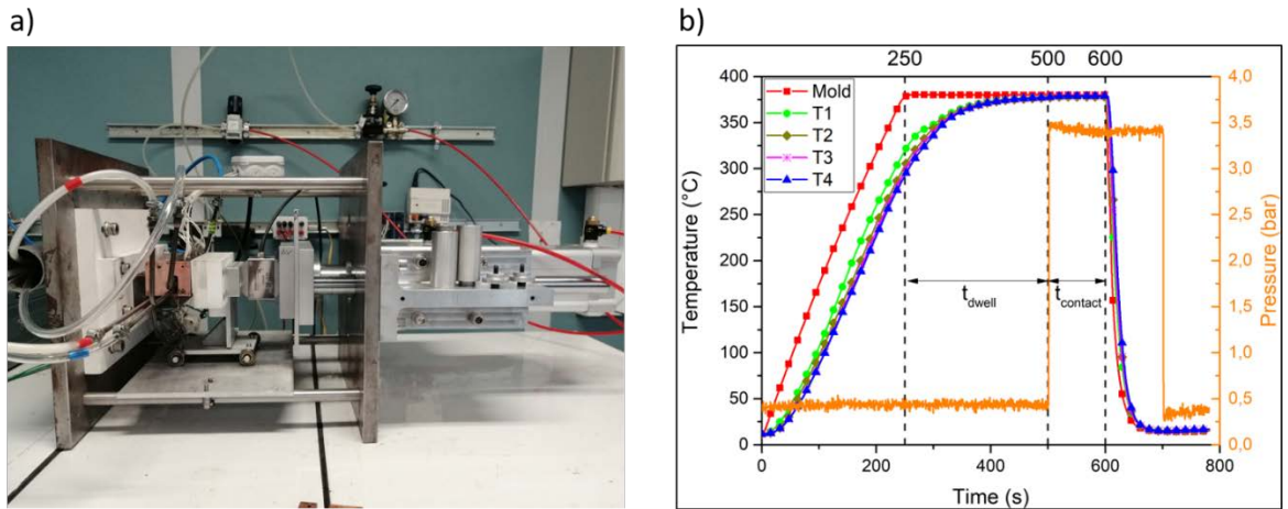
Fig. 1. (a) The TACOMA experimental welding setup and (b) the welding procedure.
