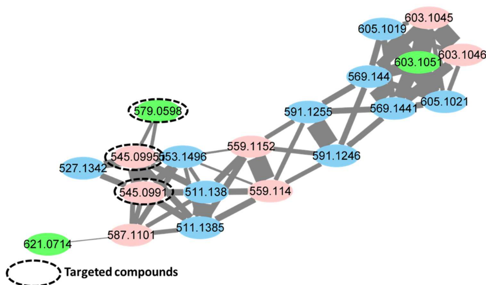
Fig. 1. Molecular family containing the new targeted chlorinated bianthrones (color-coding of the halogenation pattern is as follows: red = Cl, green = 2 x Cl).
