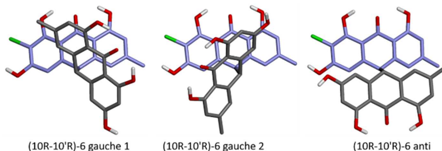
Fig. 2. Lowest-energy gauche and anti conformers of (10 R -10' R ) heterobianthrone 6 . For clarity, apolar hydrogens were omitted.
