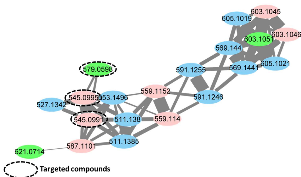
Fig. 1. Molecular family containing the new targeted chlorinated bianthrone (color-coding of the halogenation pattern is as follows: red = Cl, green = 2 x Cl).
