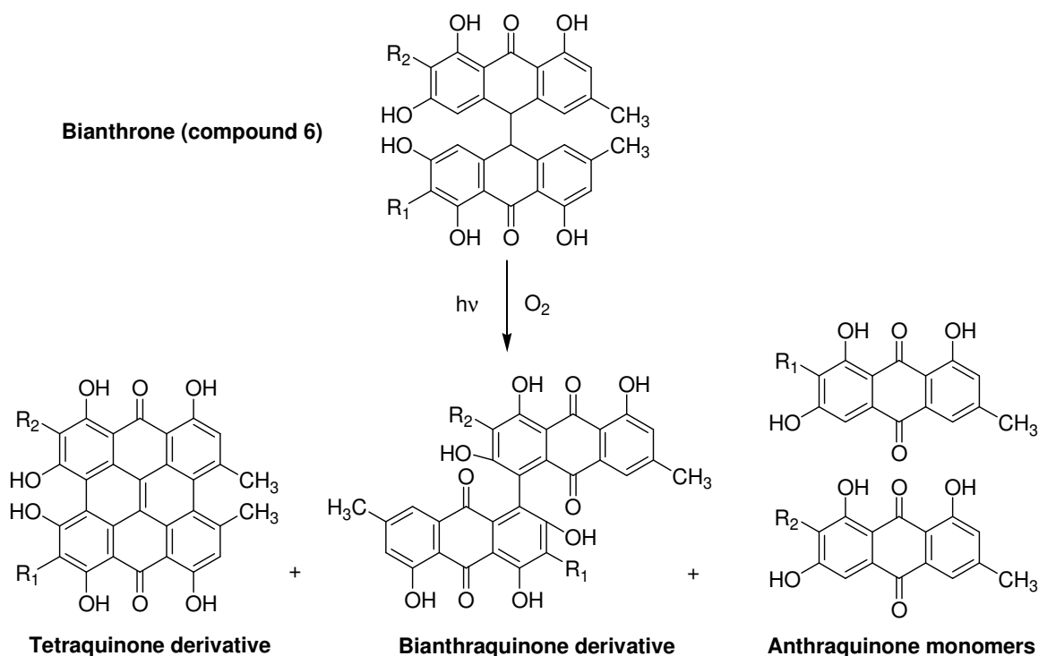
Fig. 3. Degradation products of bianthrone in presence of light and oxygen.
