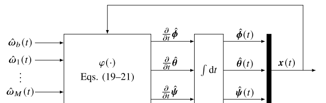
Fig. 3 Schematic of RG-WSE algorithm.
