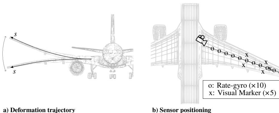
Fig. 7 Simulation wing trajectory and sensor positioning.
