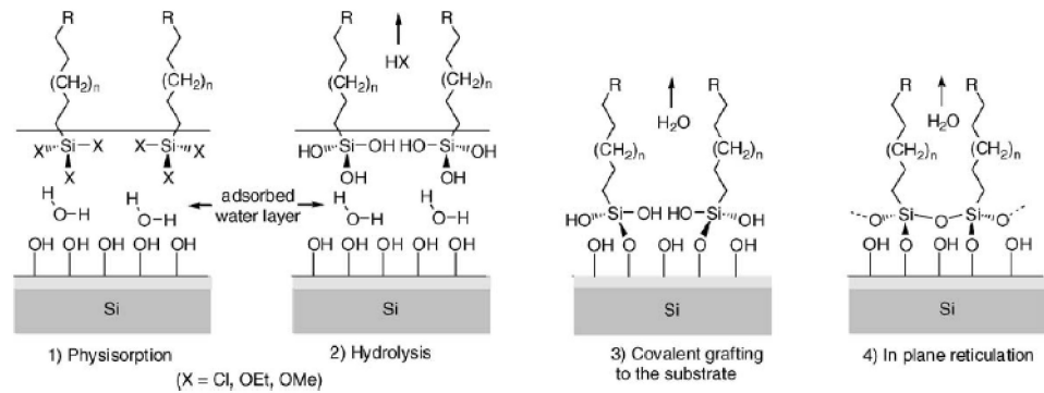
Figure 7. Silanization mechanism. Reprinted from The Lancet, 568, D.K. Aswal et al., Self-assembled monolayers on silicon. © (2006), with permission from Elsevier.
