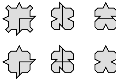
Figure 2: The six base Robinson tiles.
