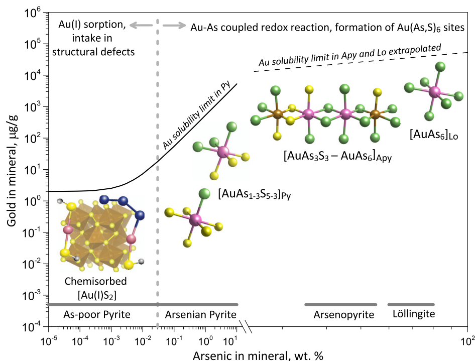
Figure 3 Structural model for chemically bound Au in pyrite, arsenopyrite and löllingite (not to scale). The Au coordination is shown by ball-and-stick atomic clusters (Au = pink, S = yellow, As = green, Fe = brown, S 3 = blue, H = grey). Horizontal gray bars indicate the typical range of As contents in each mineral. Empirical Au solubility limit in arsenian pyrite (solid curve; Reich et al. , 2005) was extrapolated to Apy and Lo (dashed curve). Note a fundamental transition in the Au incorporation mechanism (vertical dashed line, indicative position), from chemisorption as Au I -polysulfide complexes at low As content in pyrite to coupled Au-As redox reactions driving Au entry in As-enriched Fe crystallographic sites of the three minerals.
