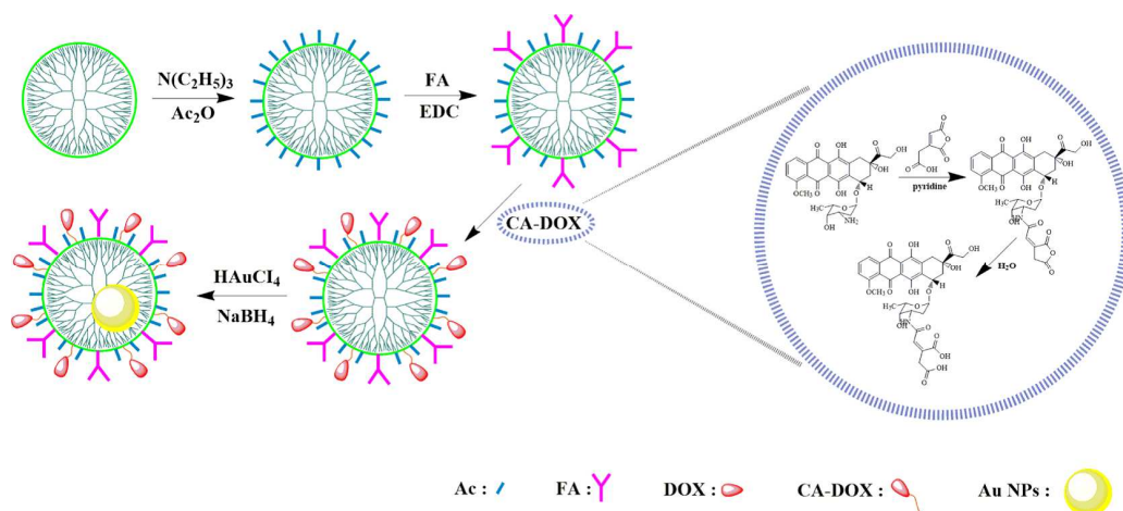
Scheme 12. Illustration of the synthesis for the pH responsive theranostic nanoplatfroms with Au encapsulating {(Au0)50-G5.NHAc-FA-DOX} (in short DOX-Au DENPs) Modified reproduction with permission from Ref. [122] Copyright 2020 ACS publications
