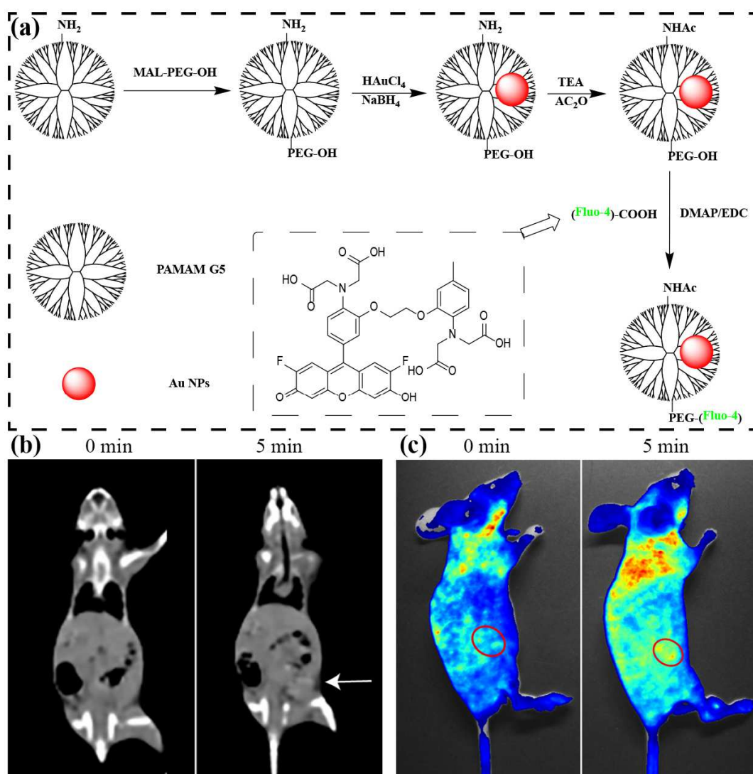
Scheme 8. Synthetic pathways for the preparation of \{(\text{Au}^0)_{25}\text{-G5.NHAc-(PEG)}_{14}\text{-(Fluo-4)}_2\} nanoprobe (a), and dual-mode CT/fluorescence images of T cells in vivo (b,c) Modified reproduction with permission from Ref. [104] Copyright 2020 ACS publications
