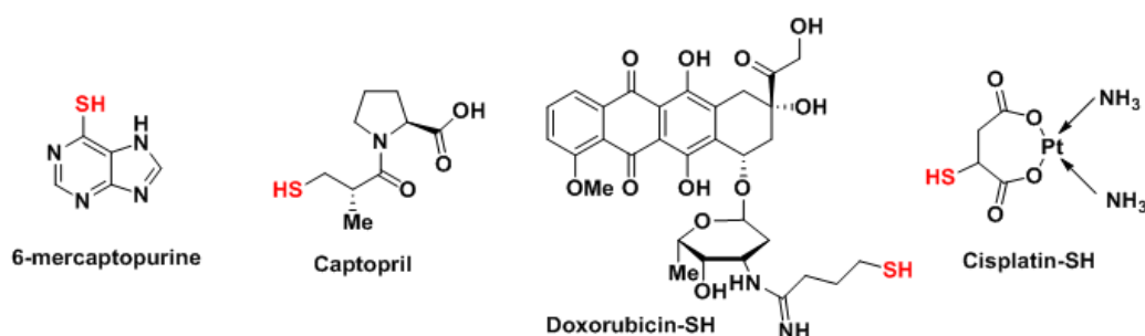
Figure 4. Representation of chemical Structures of thiol-containing (captopril and 6-mercaptopurine) and thiolated drugs (DOX and cisplatin)
