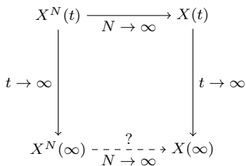
FIG 1. Illustration of the interchange of limits argument: if X^N \Rightarrow_N X and X(t) \Rightarrow_t X(\infty) , then provided technical assumptions (typically, tightness of (X^N(\infty)) ) we have X^N(\infty) \Rightarrow_N X(\infty) .
