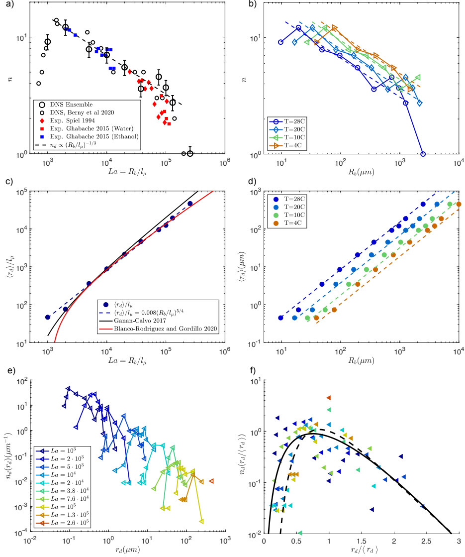
Figure 3. (a) Number of jet drops ejected, as a function of the non-dimensional bubble size R_b/l_\mu . In a) we superpose the experimental data from Spiel (1994, 1997); Ghabache (2015) for water as well as more viscous fluids allowing to explore smaller values of R_b/l_\mu (only data with Bo < 0.05 are considered to be in the regime where only R_b/l_\mu controls the drop production). Data can be described as n(R_b) = \chi \left( \frac{R_b}{l_\mu} \right)^{-1/3} . (b) Numerical data presented as a function of the dimensional R_b for 4 different water conditions, calculated from (a) using the water properties at these temperatures to compute l_\mu , showing that changes in temperature shift the drop production efficiency to larger sizes. (c) Mean ejected drop size \langle r_d \rangle / l_\mu as a function of R_b / l_\mu . The data can be described by \frac{\langle r_d \rangle}{l_\mu} = \eta \left( \frac{R_b}{l_\mu} \right)^{5/4} , close to the observed scaling for the first drop size. (d) Same data expressed in dimensional units using the water properties at these temperatures to compute l_\mu . (e) Size distribution of ejected droplets obtained for the ten ensembles considered, using l_\mu at T=28^\circ C , so that bubble radii vary from 10 to 2400 \mu m . The distribution of ejected droplet size varies from 0.1 to 100 \mu m . (f) Normalized distributions, with a Gamma distribution of order 4 superimposed (solid black line) and a log-normal distribution (dashed black line).
