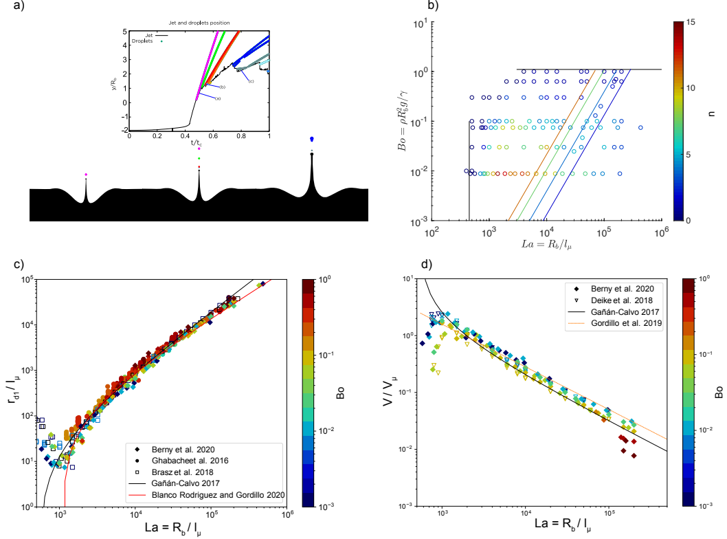
Figure 1. Jet drop dynamics and characteristics. (a) Numerical simulations of the two-phase flow process can be performed, and capture for a given initial cavity all jet drops being produced (Bery et al., 2020). Inset shows the position of the tip of the jet (black) and droplet position (the ejected drop being color-coded). (b) Phase diagram of existence of jet drops in terms of controlling parameters, R_b/l_\mu and R_b^2/l_c^2 , from Bery et al. (2020). The number of ejected droplet is color-coded. The colored lines correspond to salt water conditions at 4, 10, 20 and 28°C. For R_b^2/l_c^2 > 1 , no jet drops are being produced. (c) The first drop size, normalized by the visco-capillary length, r_{d1}/l_\mu , as a function of the normalized bubble size R_b/l_\mu . The first drop size can be described by a universal scaling (eq. 3) and all data collapse onto a single curve. Symbols are simulations and laboratory experiments from Ghabache et al. (2016); Brasz et al. (2018); Deike et al. (2018); Bery et al. (2020). (d) Same data for the jet drop velocity V/V_\mu as a function of R_b/l_\mu . Again, all data collapse onto a single curve and can be described by a universal scaling (eq. 2).
