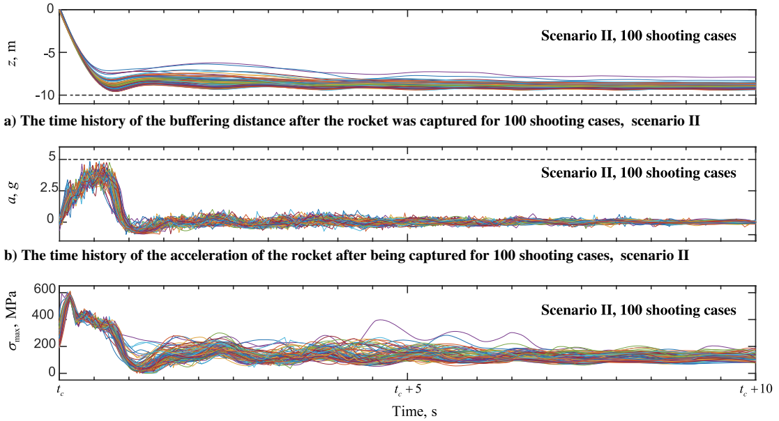
c) The time history of the maximum stress on the cables after the rocket was captured for 100 shooting cases, scenario II
