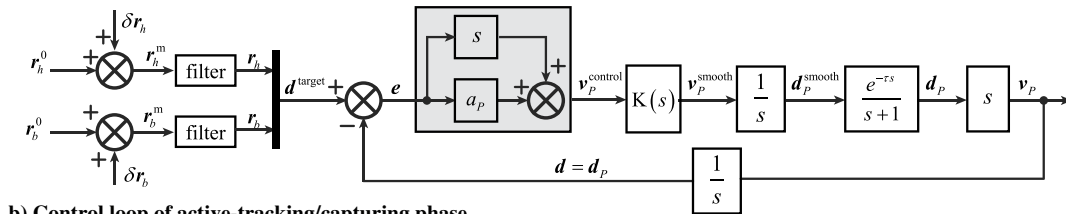
b) Control loop of active-tracking/capturing phase
