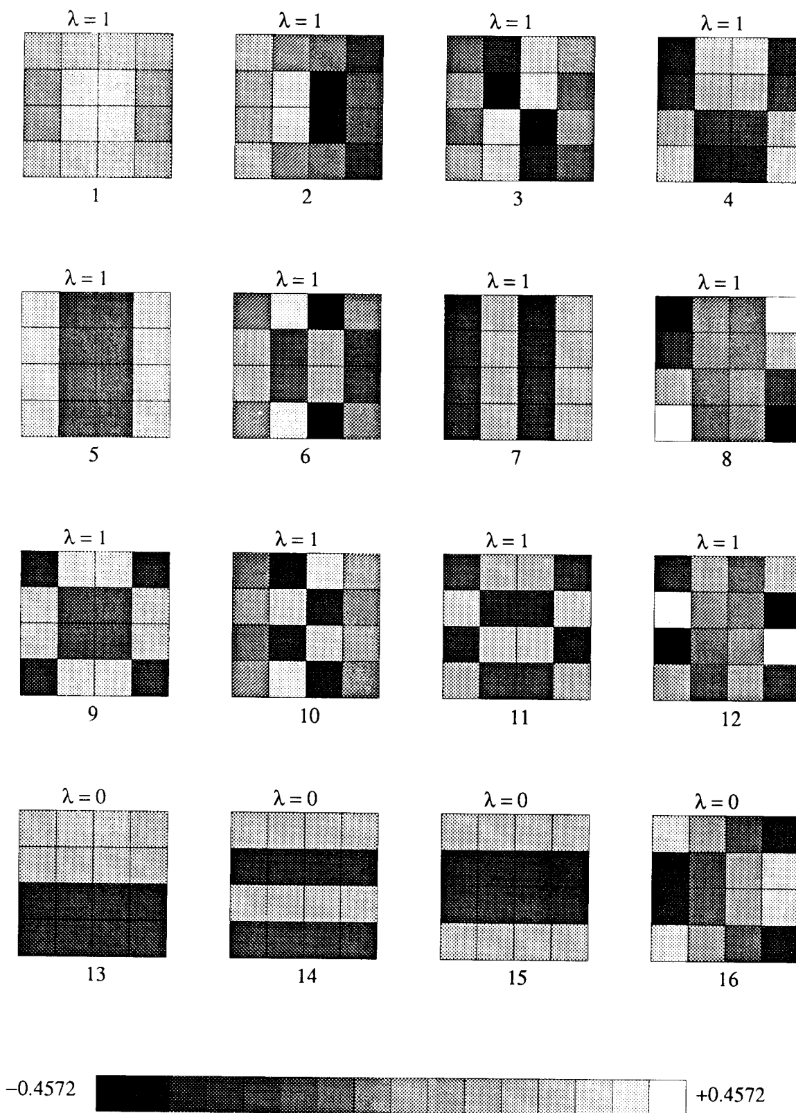
Figure 4. Eigenvectors of the resolution operator associated with the experimental geometry shown in Fig. 1 and with the Lanczos's inversion operator. The first 12 eigenvectors correspond to the degenerate eigenvalue equal to 1. The last four eigenvectors correspond to the degenerate zero eigenvalue. The grey scale is common to the 16 normalized eigenvectors; minimum and maximum values of their components correspond to black and white, respectively.
