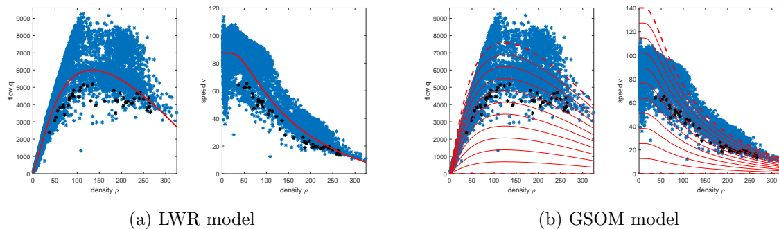
Figure 5: Fundamental flow and speed diagrams for RTMC data corresponding to loop S1708 . In red, equilibrium curve for LWR (Figure 5a) and family of flow and speed curves for GSOM (Figure 5b) based on the optimal calibration parameter of Table 2. In black: data of the selected scenario (see Figure 3b).
