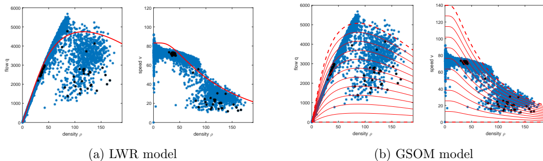
Figure 4: Fundamental flow and speed diagrams for DirMed data corresponding to loop 303. In red, equilibrium curve for LWR (Figure 4a) and family of flow and speed curves for GSOM (Figure 4b), based on the optimal calibration parameters of Table 2. In black: data of the selected scenario (see Figure 3a).
