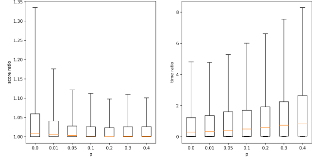
Figure 5: The ratio of the best fitness (left) and the run time (right) of the SAP-EA with \mu = 1 , \alpha = 0.4 , \beta = 35 , and different values of p compared to the SAP-B. The run times of SAP-B range from 0.3 seconds to 30 minutes, with better time ratios for higher SAP-B run times. Each boxplot contains the data of all 20 runs per value of k and per each of the 25 scenarios, totaling to 2000 points per box. The orange line depicts the median, the box the mid-50 % of the data, and the whiskers the mid 95 %. A higher value of p , i.e., an increased use of RandomPwD, yields generally better solutions and a smaller spread but also increases the run time. A sweet spot seems to be around p = 0.05 . Please also refer to Section 5.2.2.
