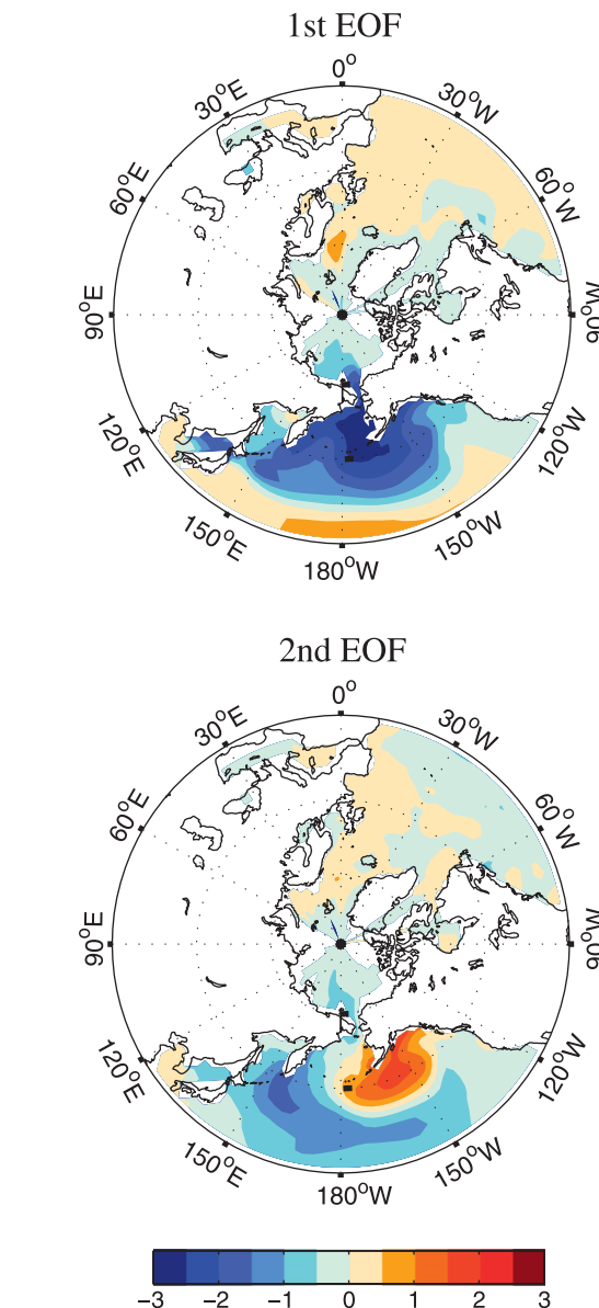
FIG. 6. First and second leading EOFs of surface \Delta^{14}\text{C} in the northern extratropics, accounting for 36% and 19% of the variance, respectively; EOFs calculated as in Fig. 3.
