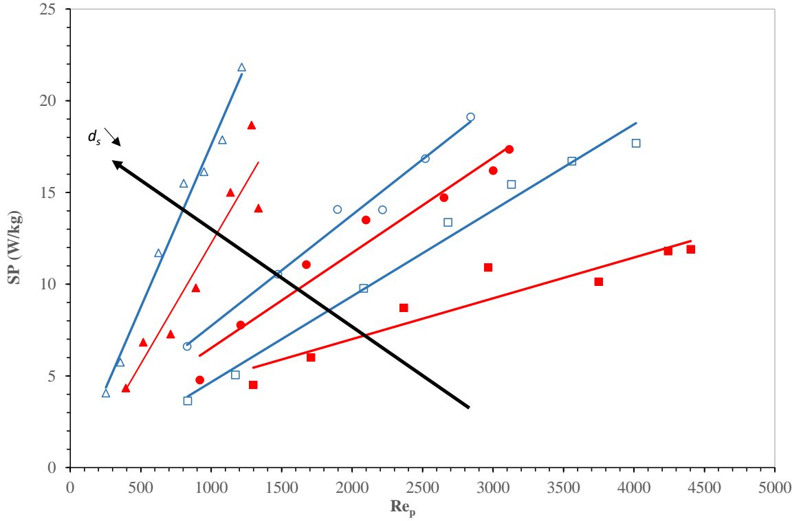
Figure 9: Mass-specific power vs. pore Reynolds number for the various packed bed arrangements Full symbol: Charging cycle - Empty symbol: Discharging cycle - Square: D/d_s = 3.11 - Circle: D/d_s = 4 - Triangle: D/d_s = 9.3 .
