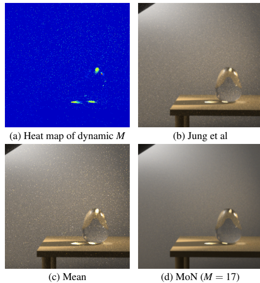
Figure 5: Jung et al dynamic M map overview at 10,000 samples on cropped part of Veach scene with visual results of Jung et al, mean and MoN final estimators. The heat map is composed of possible values of M ranging from 1 to 17.
