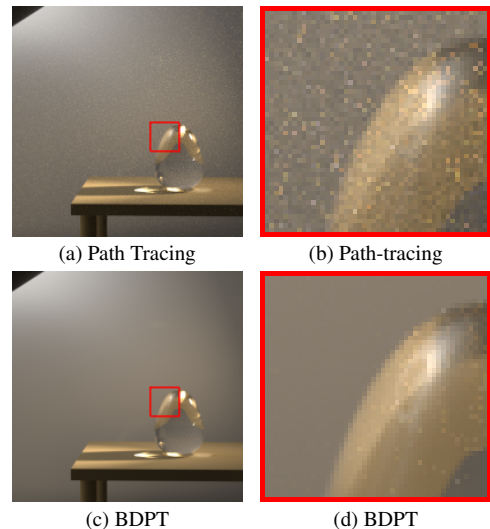
Figure 2: Fireflies overview on cropped part of Veach scene using Path Tracing and BDPT with 100,000 samples for each.
