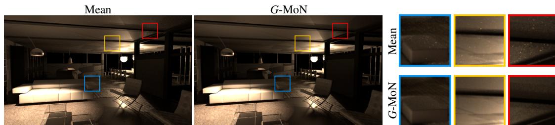
Figure 1: Comparison of G -MoN (adaptive Median of meaNs with use of the Gini coefficient) and classical mean estimators on Villa scene with 100,000 samples using Path Tracing for each. The mean even at 100,000 samples is still sensitive to the high contributions while this estimator remove the whole fireflies present in the image.
