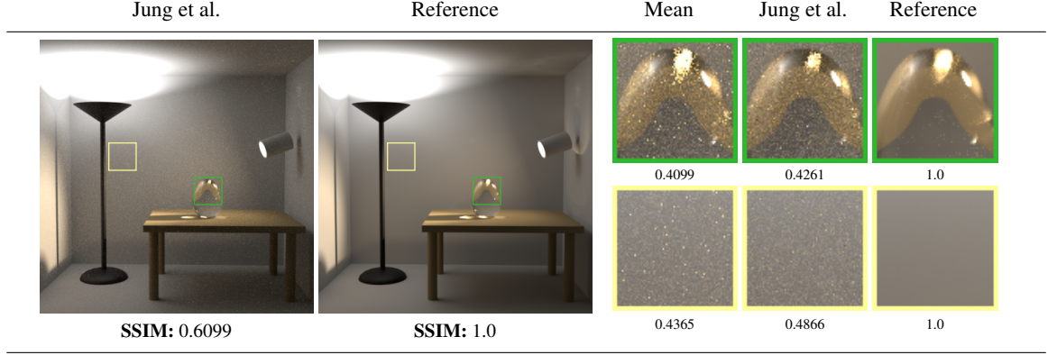
Figure 6: Comparison of classical Mean, Jung et al with automated M and reference using BDPT images obtained with 10,000 samples per pixel.
