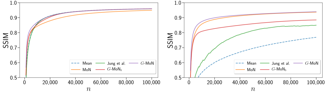
(a) Comparisons of 5 estimators using SSIM during rendering on the Bathroom image. (b) Comparisons of 5 estimators using SSIM during rendering on the Veach image.
